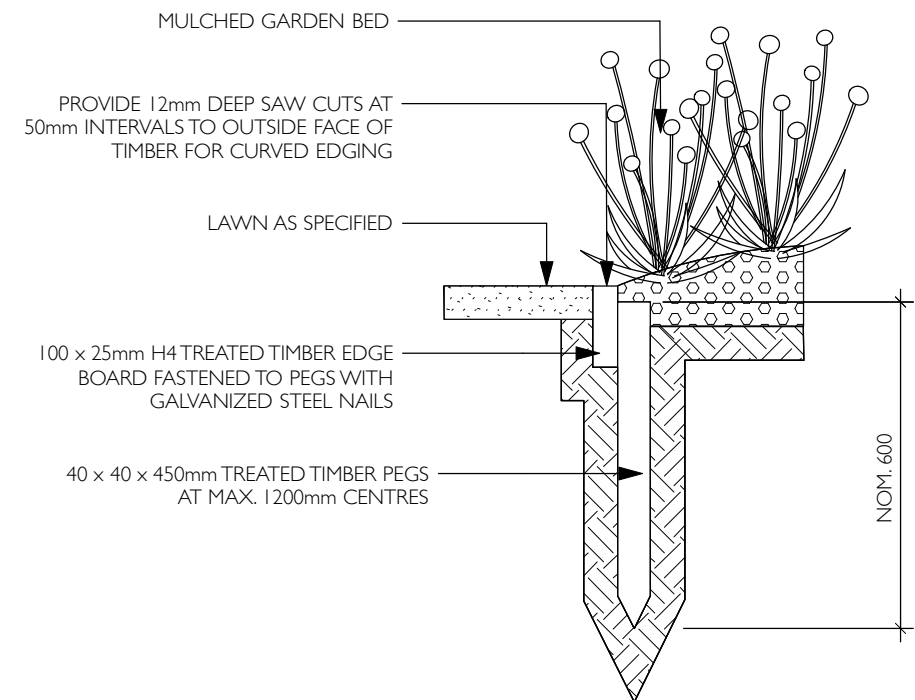
TYPICAL TIMBER LAWN EDGING DETAIL SCALE 1:50
