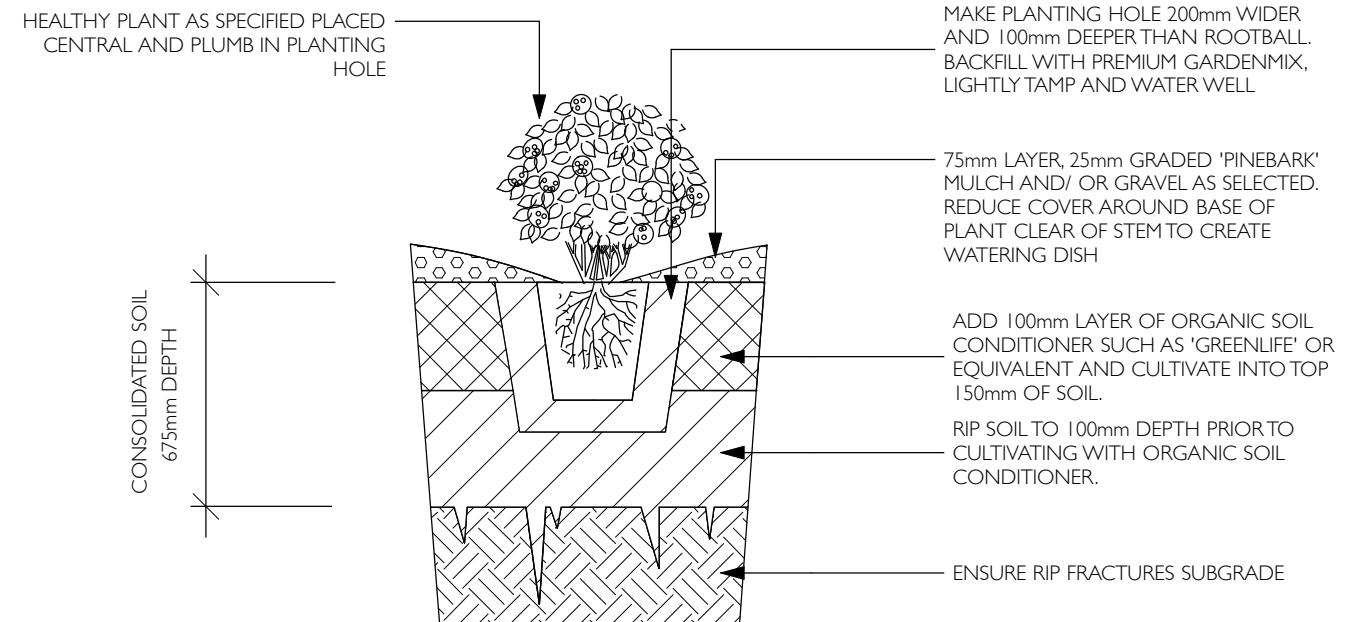
TYPICAL PLANTING DETAIL SCALE 1:20
